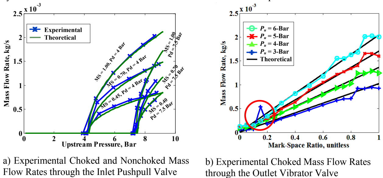
Figure 3 –Flow Characterization of the Actuator
