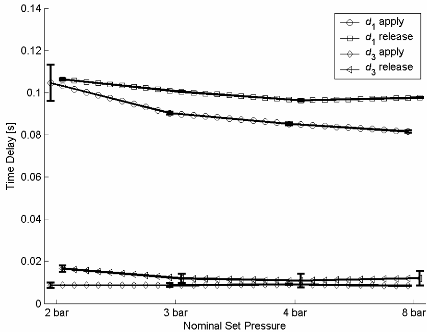
Figure 11. Time Delays
