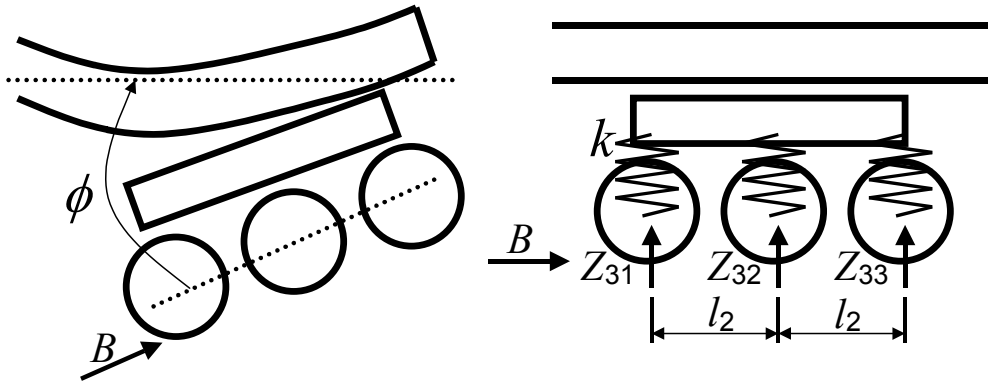
Figure 5. Chassis Compliance
