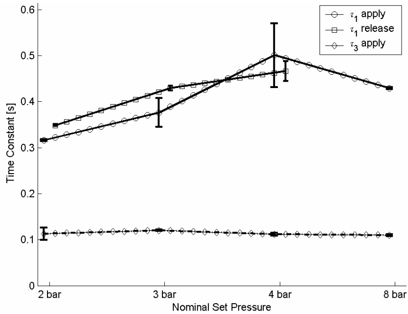
Figure 12. Time Constants
