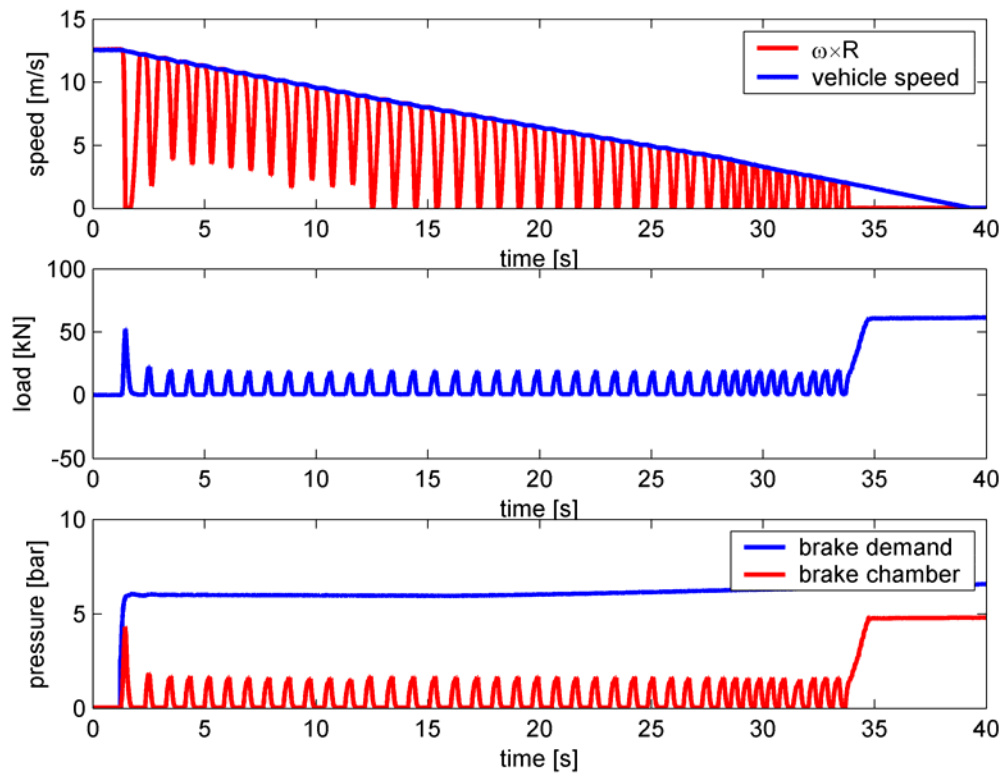
Figure 1 HIL Results \mu=0.20
