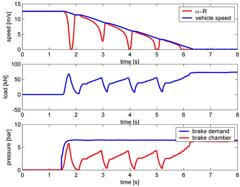
Figure 3 HIL Results \mu=0.75
