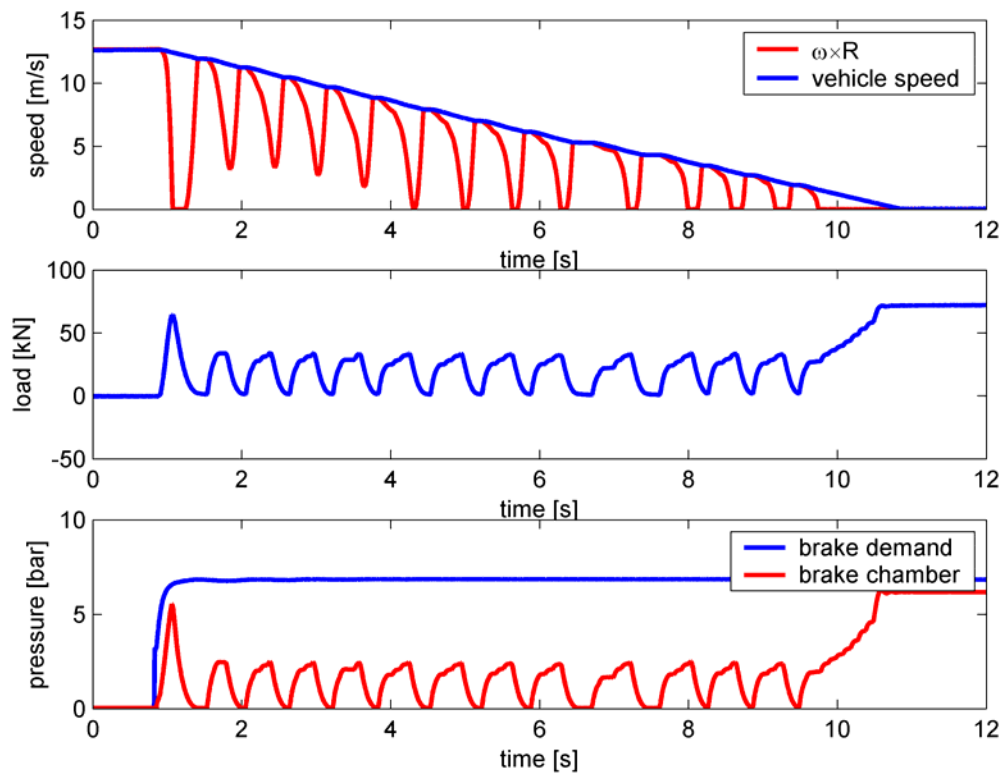
Figure 2 HIL Results \mu=0.40
